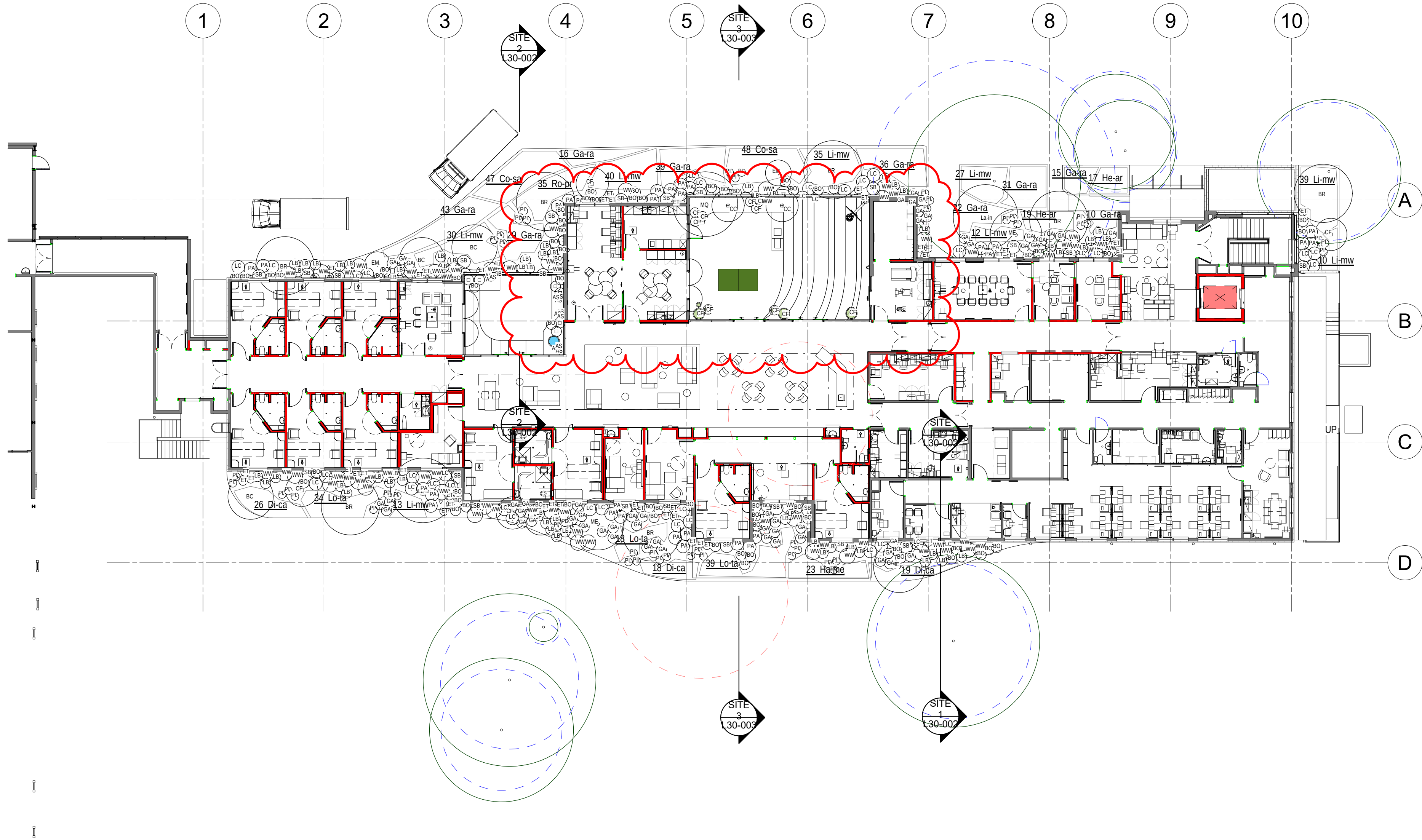
1 LEVEL 1 PLANTING PLAN 1 : 200
